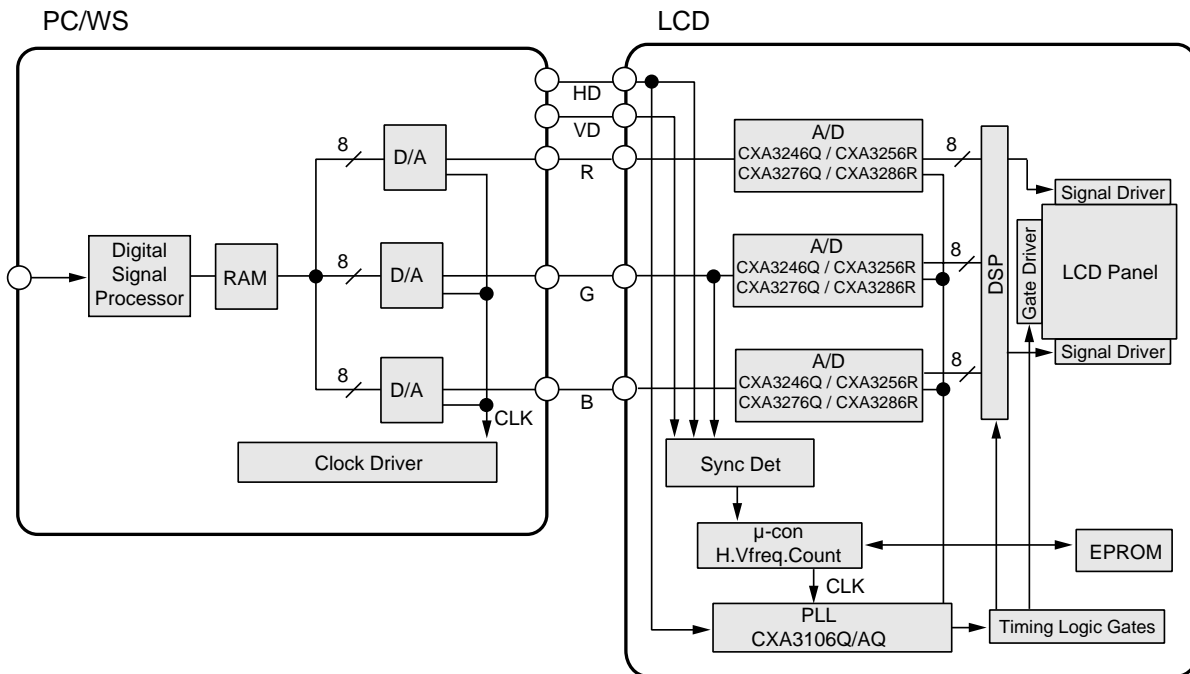
LCD Monitor System Block Diagram
